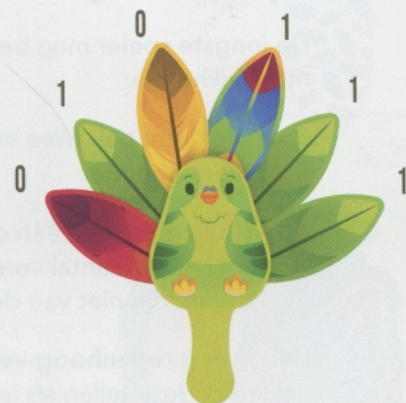
Example Scoring
